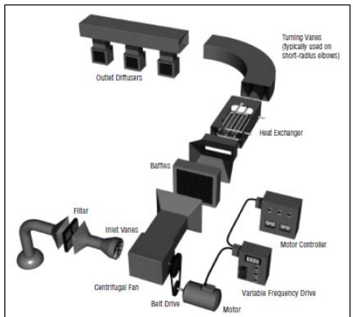
Figure 1. Example of fan system components. 1 Illustration from Lawrence Berkeley National Laboratory
